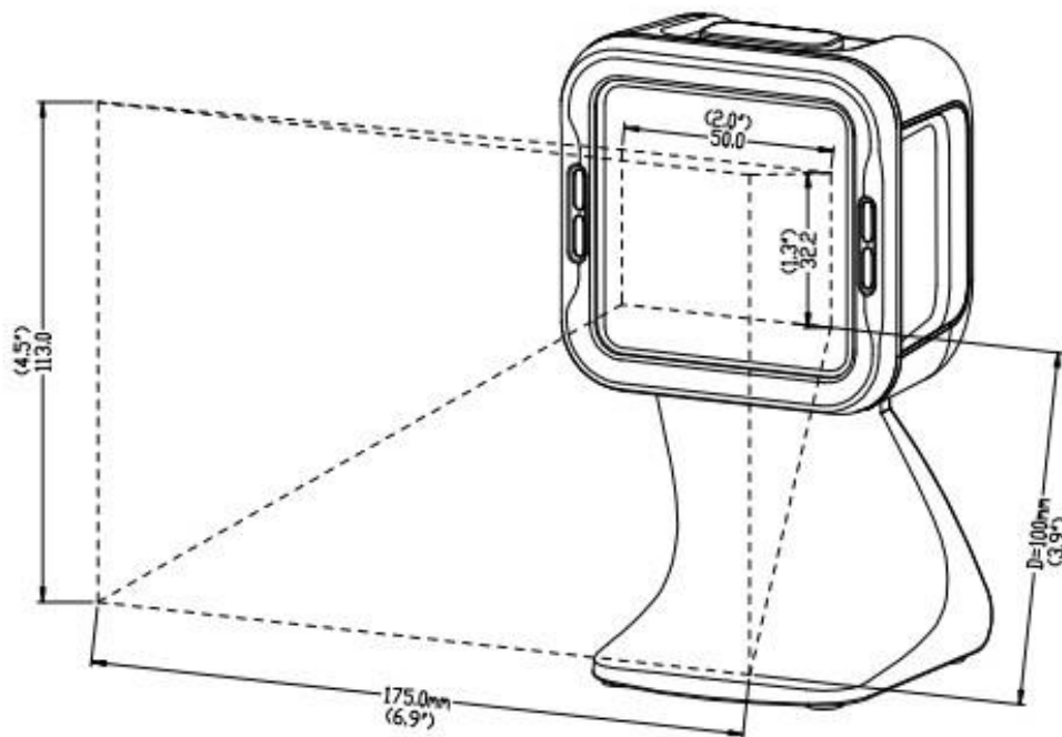
Figure 2-6 Field of view
