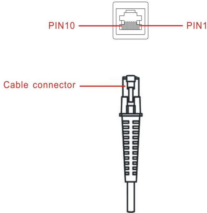
Figure 2-1 Cable connector interface pin-outs
