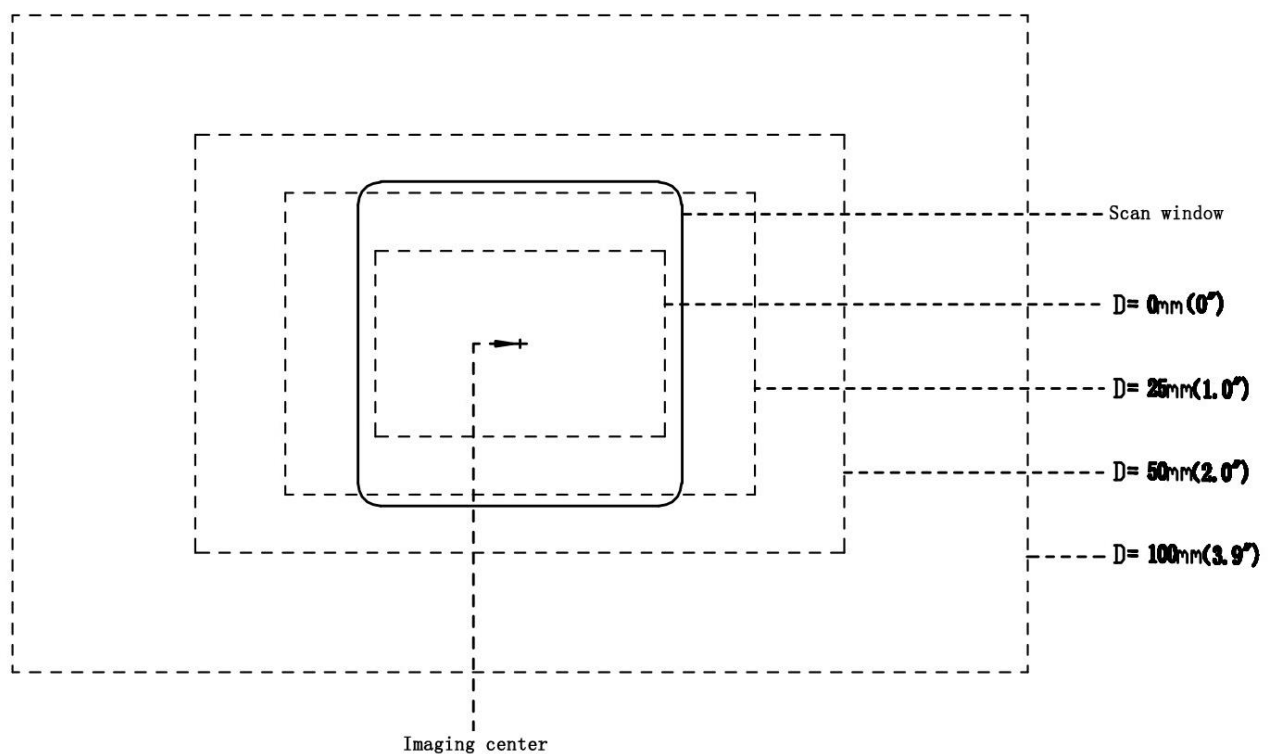
Figure 2-7 Field of view - Front view
