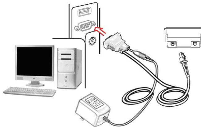
Figure 2-6 Installation of RS232 cable
