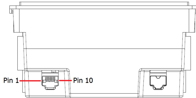
Figure 2-1 Cable connector interface pin-outs
