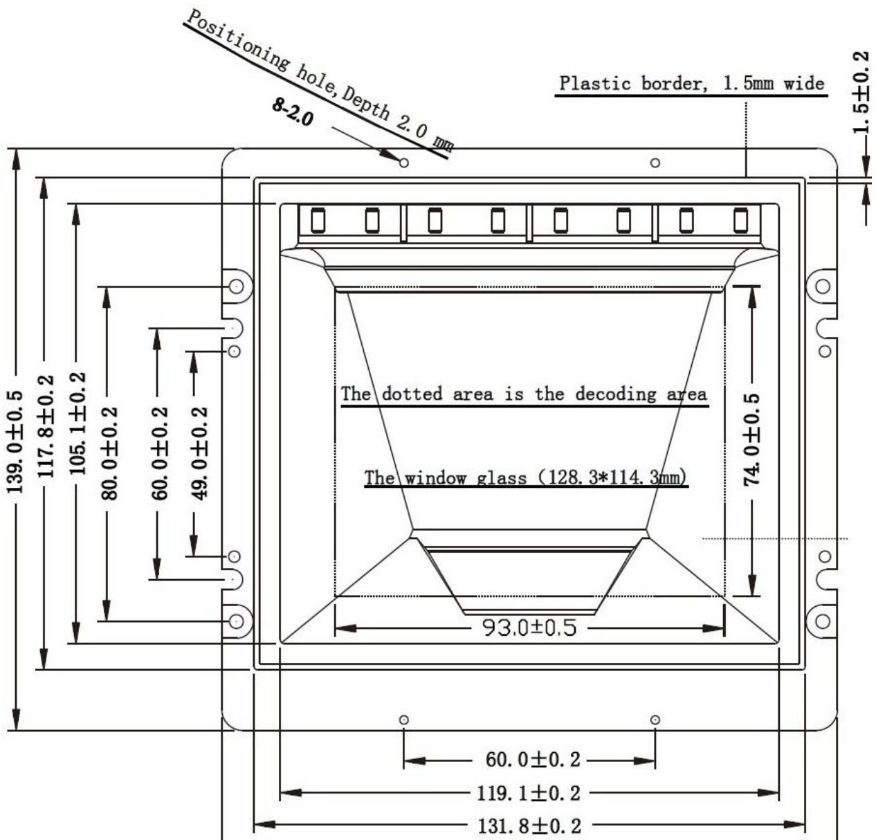
Figure 2-2 Dimensions (without stand)
