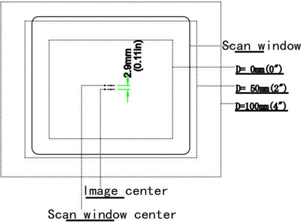
Figure 2-5 Field of view – Front view
