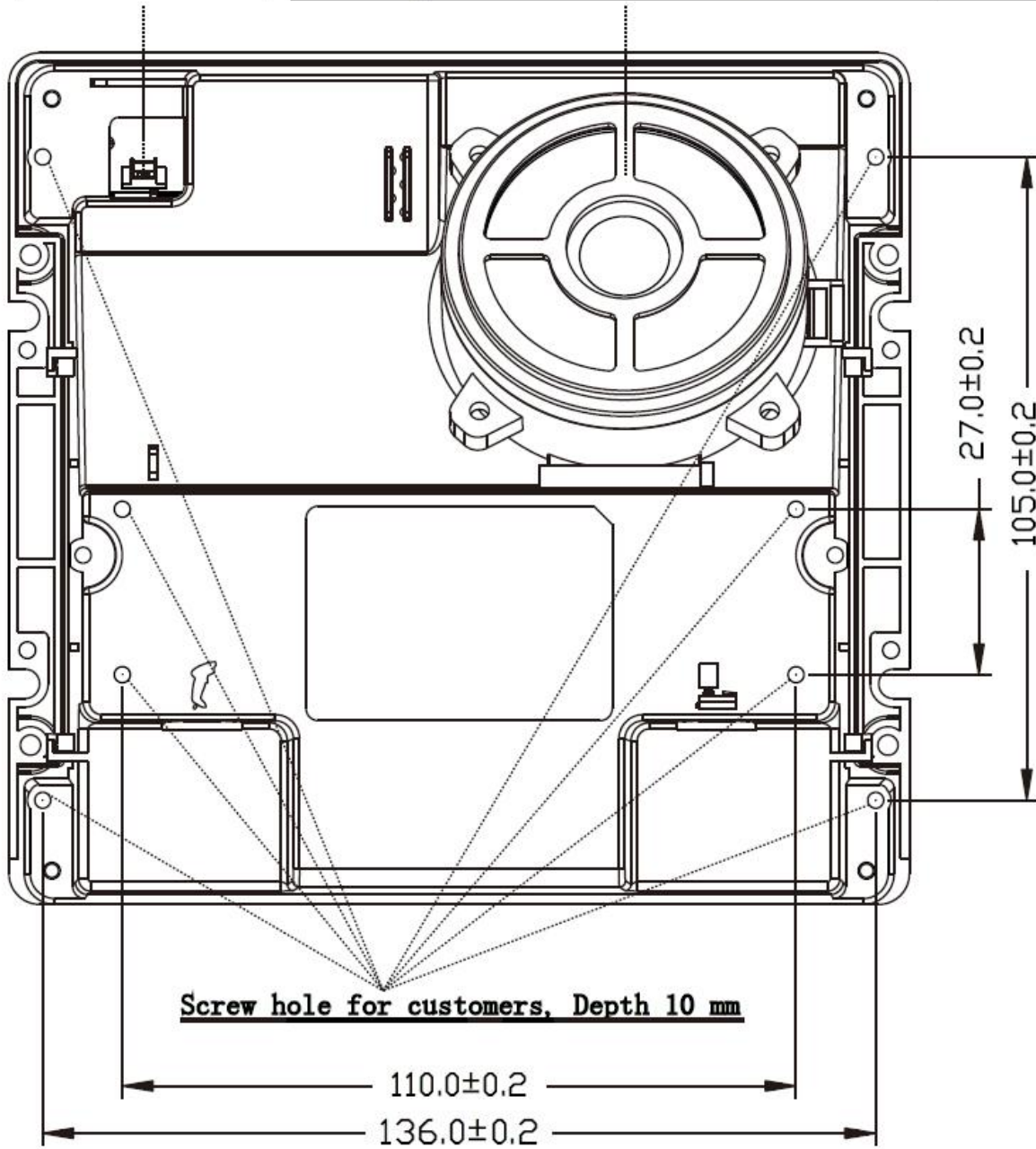
Figure 2-4 Dimensions of hanging holes
