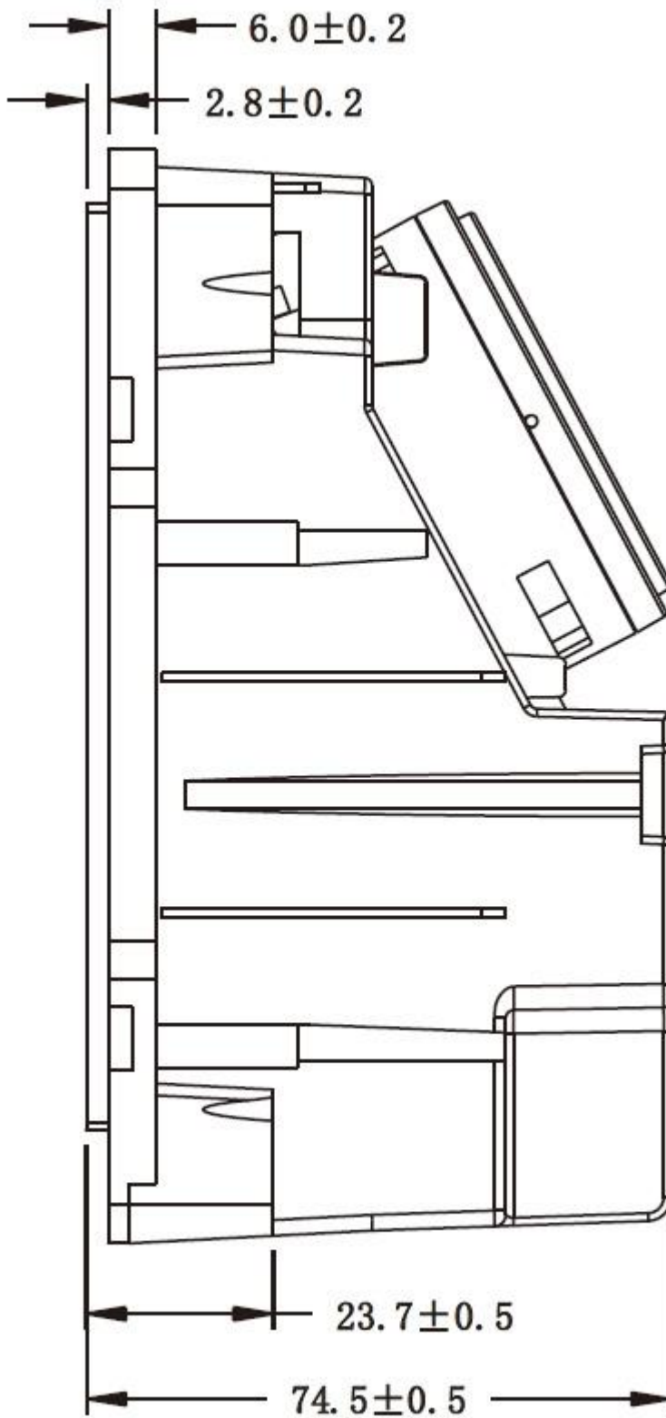
Figure 2-3 Dimensions (with stand)
